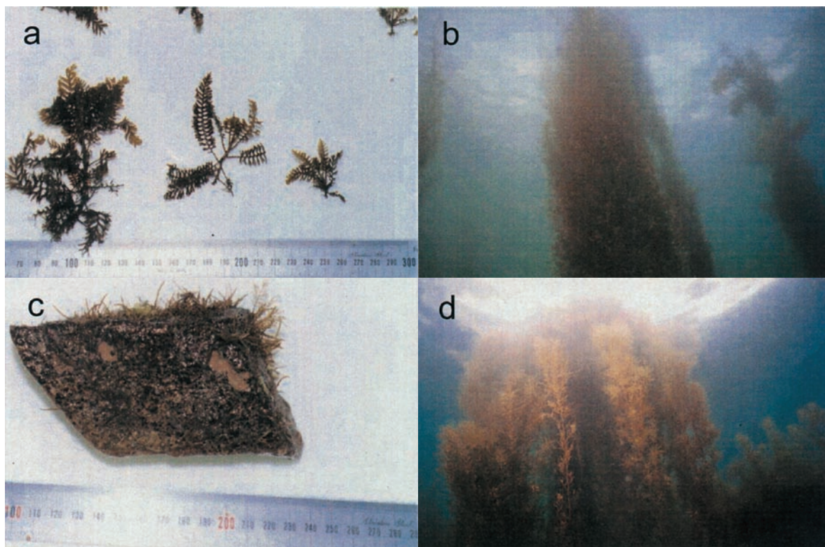
Fig. 6. Seasonal changes in plant appearance of S. horneri at the two habitats in Hiroshima Bay. Plants at the Ohno habitat in August (a), December (b), at the Ihota habitat in July (c), March (d).
