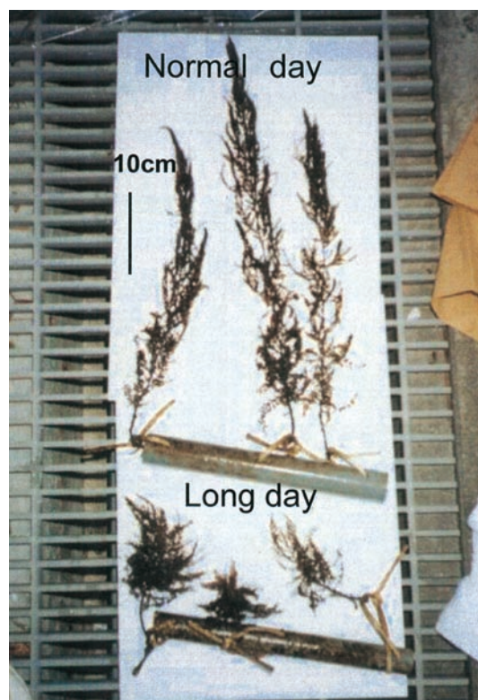
Fig. 34. The St. 5 plants cultured in the outdoortanks under the natural (upper three plants) and the artificial-long day condition (lower three plants) in January 2002.
