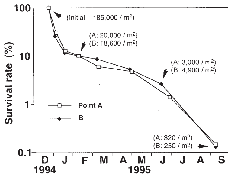
Fig. 42. Survival rate of the S. horneri embryos settled on the artificial substrata set at the two points in the St.1 community. Numbers in parenthesis indicate individual density on the substrata.
