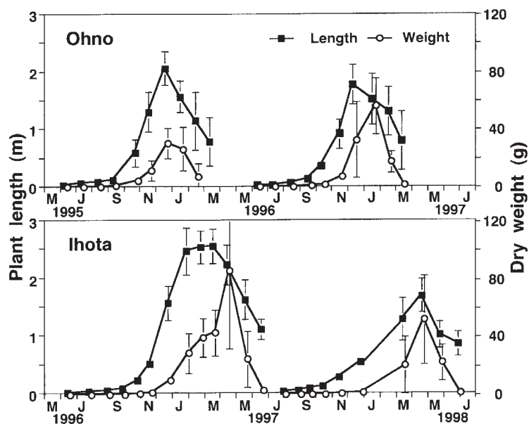
Fig. 3. Seasonal change of plant length and dry weight of the two S. horneri populations in Hiroshima Bay. Data are means with S.D. for the ten largest plants in length at each survey.
