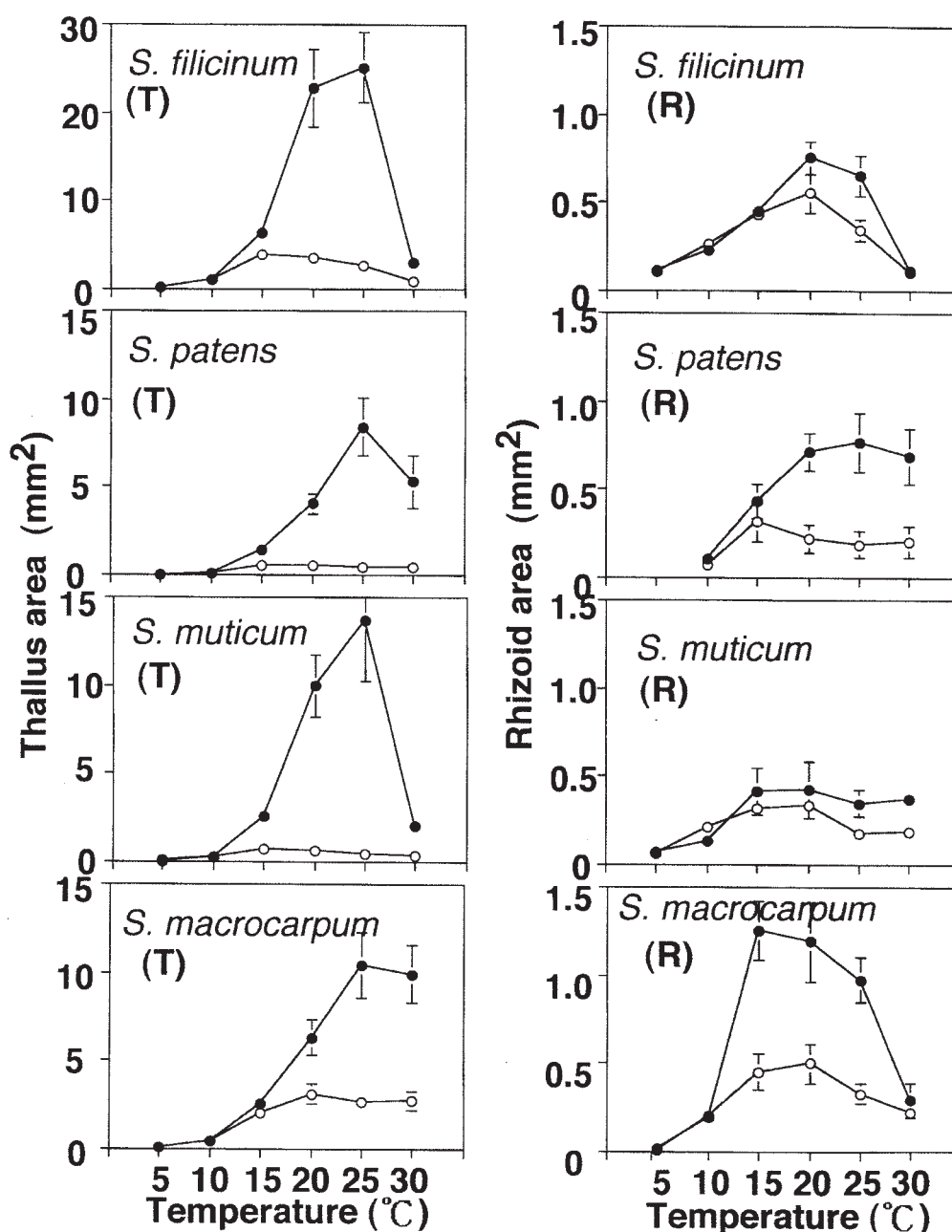
Fig. 21. Thallus (T) and rhizoid (R) area of young plants of four Sargassum species cultured under various temperature conditions for 4 weeks. At 80 \mu \text{Em}^{-2} \text{s}^{-1} (●) and 25 \mu \text{Em}^{-2} \text{s}^{-1} (○).
