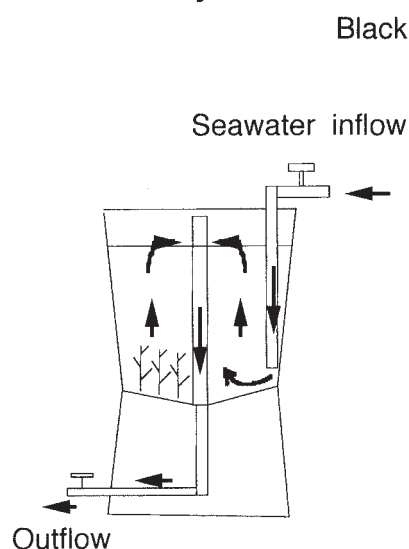
Fig. 24. The experimental system of the outdoor culture experiments on the effects of natural and artificial-long day conditions on the growth of S. horneri plants.
