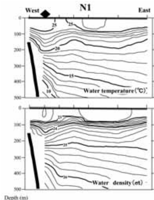
Fig. 2-4. Vertical profiles of water temperature (°C) and density ( \sigma_t [kg/m 3 ]) across the Kuroshio Current obtained during the research cruise of Soyo-Maru in November, 2000. Measurements were performed at N1 line. See Table 2-1 and Fig. 2-3 for detail. ◆ indicates the position of an axis of the Kuroshio. Thick solid lines indicate sea bottom.
