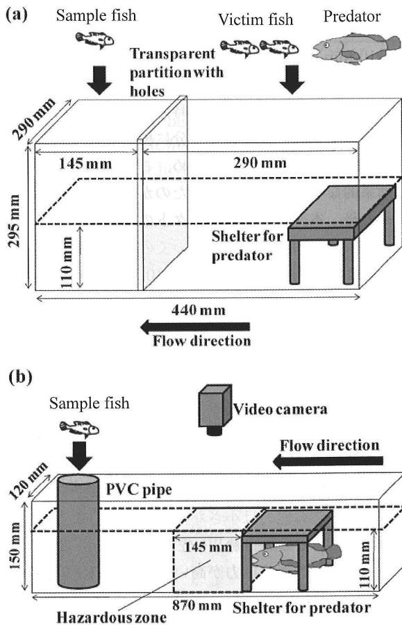
Fig. 13. Schematic drawings of the experimental tanks: (a) the experiencing tank and (b) the behavioral observation tank. The sample black-spot tuskfish ( Choerodon schoenleini ) in the behavioral observation tank was the fish that had been conditioned in the experiencing tank. The PVC pipe in the behavioral observation tank was removed when the observation was started. Redrawn after Kawabata et al. (2011b) with permission.
