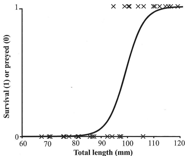
Fig. 5. Relationship between body size and survival of black-spot tuskfish ( Choerodon schoenleinii ) in the laboratory experiment. Survival and death of the fish are plotted as 1 and 0, respectively, by X. The logistic curve for the survival probability in relation to tuskfish size is shown. The size at 50% survival was estimated to be 98 mm in total length (TL). Redrawn after Kawabata et al. (2011a) with permission.
