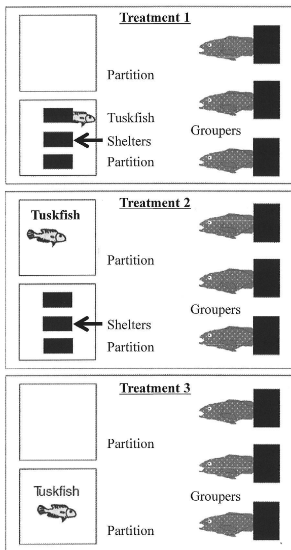
Fig. 9. A schematic drawing of the overhead view of the three treatments. Treatment 1 (top): black-spot tuskfish ( Choerodon schoenleinii ) were acclimated to shelters prior to exposure to white-streaked groupers ( Epinephelus ongus ). Treatment 2 (middle): black-spot tuskfish were not acclimated to shelters but shelters were available during exposure to groupers. Treatment 3 (bottom): black-spot tuskfish were not acclimated to shelters and no shelters were available during exposure to groupers. Partitions were removed at the start of the experiment. Redrawn after Kawabata et al. (2011a) with permission.
