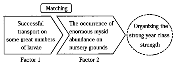
Fig. 3. Matched factors organizing the strong year class strength of Japanese flounder in the Northern Pacific.
