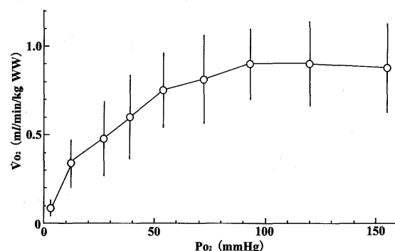
Fig.2 Change in the amount of oxygen uptake ( \dot{V}_{O_2} ) with decreasing the oxygen tension ( P_{O_2} ) in S. virgatus . Circles and vertical lines are the mean values and the standard deviations, respectively.
