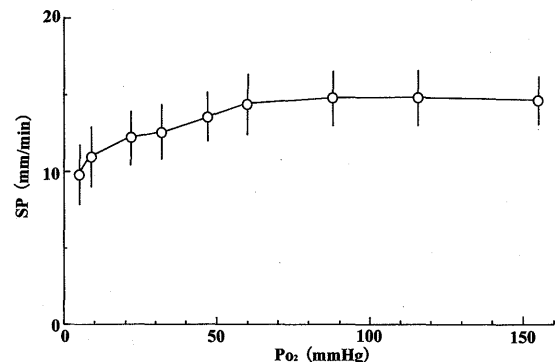
Fig. 5 Change in the moving speed of vinyl film (2.0 mm diameter, 0.3 mm thickness) on the gill surface (SP) in S. virgatus with decreasing the oxygen tension ( P_{O_2} ). The symbols are the same as those in Fig. 2.
