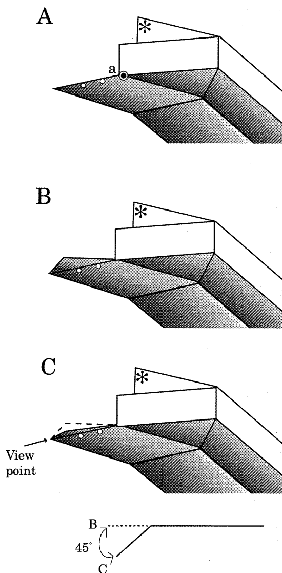
Fig. 5. The structure of the floor of the terminal edge of the fishway in experiment II-B and II-C. A, trapezoid in dorsal view; B, triangle; C, triangle ( -45^\circ on tip). Explanations of symbols are the same as shown in Fig. 3.
