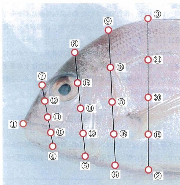
Fig. 1. Landmarks on a fish.
