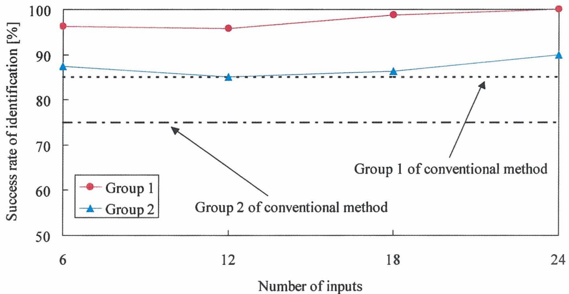
Fig. 10. Success rates of identification.
