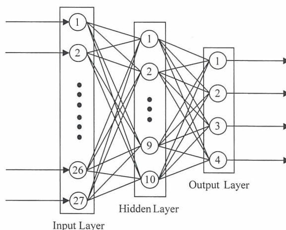
Fig. 2. Layered neural network for 27 color data.
