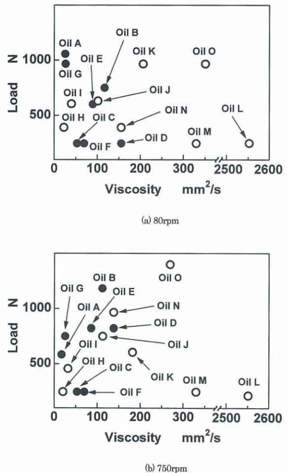
Fig. 7. Relationships between viscosity and seizure load
