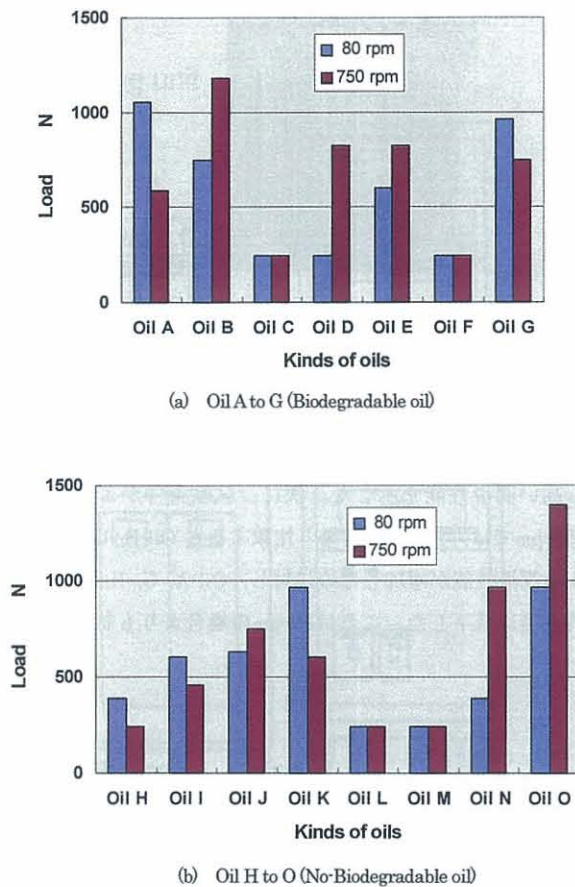
Fig. 6. Results obtained from Four-ball test
