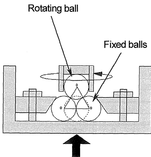
Fig. 2. Test balls setting configuration
