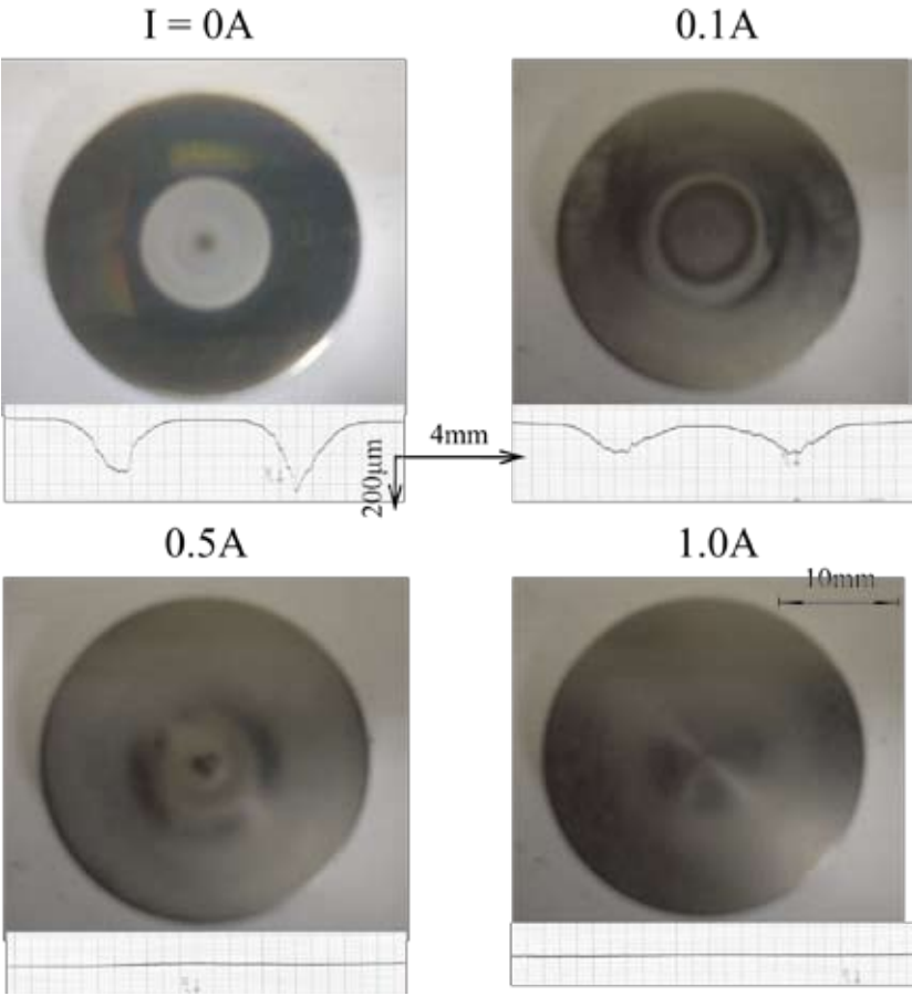
Fig. 8. Aspects of the eroded area under cathodic protection for Ti-6Al-4V ( t=10 h).
