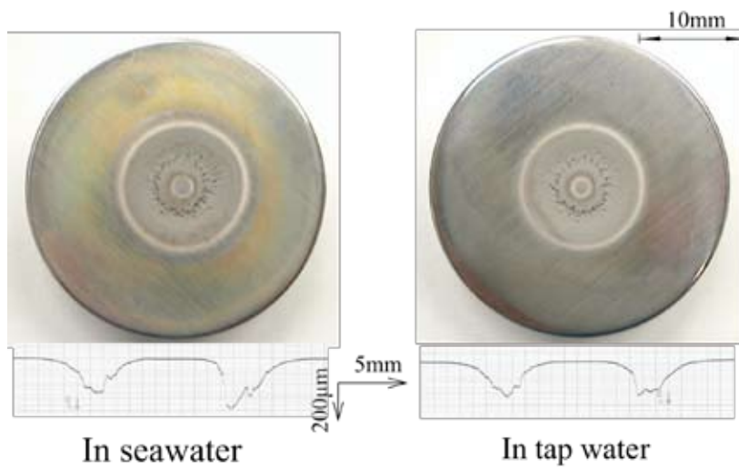
Fig. 5. Aspects of eroded area in seawater and tap water for Ti-6Al-4V ( t=15 h) .
