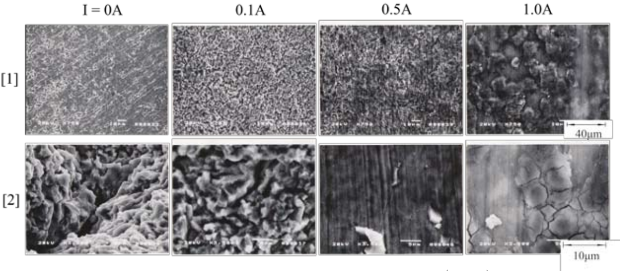
Fig. 9. SEM photographs of the eroded surfaces for Ti-6Al-4V ( t=10 h). [1] around the ring-like erosion ; [2] near the point of severe erosion.
