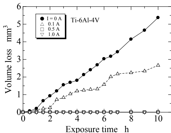
Fig. 7. Volume loss versus exposure time and cathodic current.
