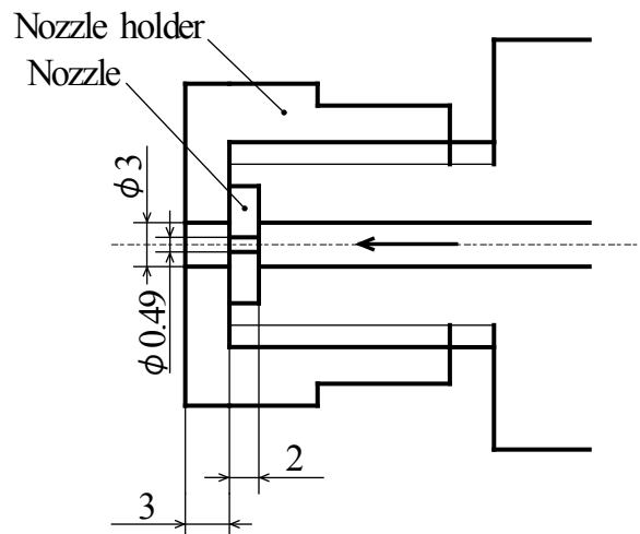
Fig. 2. Test nozzle and holder.
