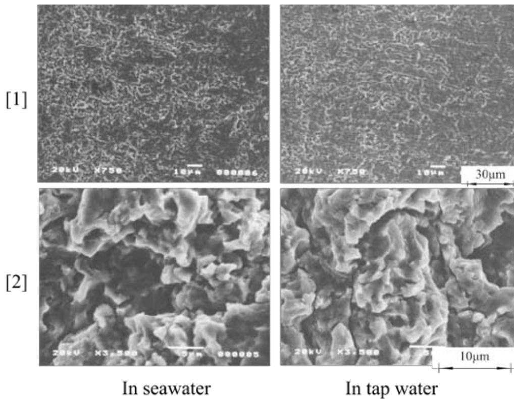
Fig. 6. SEM photographs of the eroded surfaces for Ti-6Al-4V. [1] around the ring-like erosion ; [2] near the point of severe erosion.
