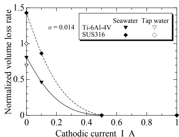
Fig. 10. Relation between the normalized volume loss rate and cathodic current.
