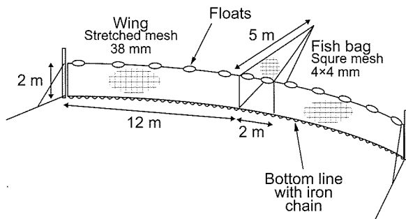
Fig. 2. Diagram of the experimental beach seine YS Surf-net.
