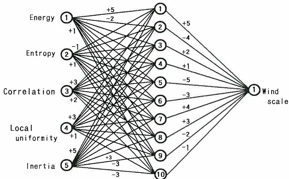
Fig. 3. The Structure of neural network after leaning
