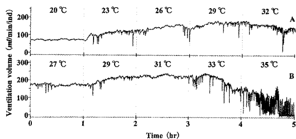
Fig.2. Ventilation volume ( V_g ) in the black-lip pearl oyster recorded with rising the water temperature. Numeral in upper figure, water temperature; A, rise from 20.0 \pm 0.1 ^{\circ}\text{C} at the rate of 3 ^{\circ}\text{C/hr} ; B, rise from 27.0 \pm 0.1 ^{\circ}\text{C} at the rate of 2 ^{\circ}\text{C/hr} .
