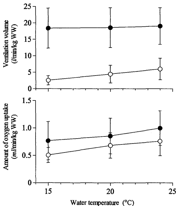
Fig.1. Changes in ventilation volume and amount of oxygen uptake in the Mediterranean blue mussel Mytilus galloprovincialis with feeding Chaetoceros gracilis (20,000 cells/ml) at 15.0 \pm 0.5^\circ\text{C} , 20.0 \pm 0.6^\circ\text{C} and 24.0 \pm 0.6^\circ\text{C} . Circles and vertical lines show mean and standard deviation, respectively. Open circle, before feeding; closed circle, during feeding; WW, wet weight of soft part of body.
