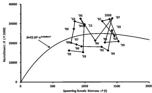
Fig. 5. Stock-recruitment relationship of yellow sea bream.
