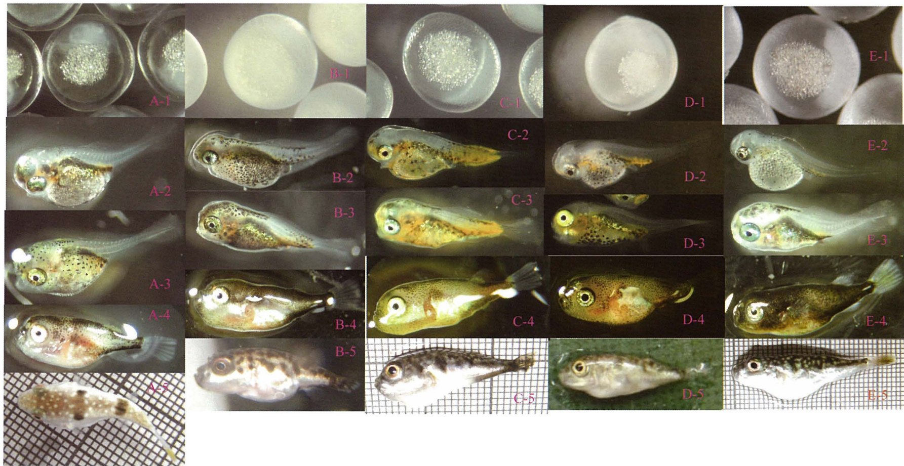
Fig. 2. Photos of eggs (1), hatched larvae (2), post larvae (3), juveniles (4) and young fishes (5) of Takifugu niphobles (A), T. pardalis (B), T. poecilonotus (C), T. snyderi (D) and T. stictonotus (E). Age in days and standard length are shown in Table 2.
