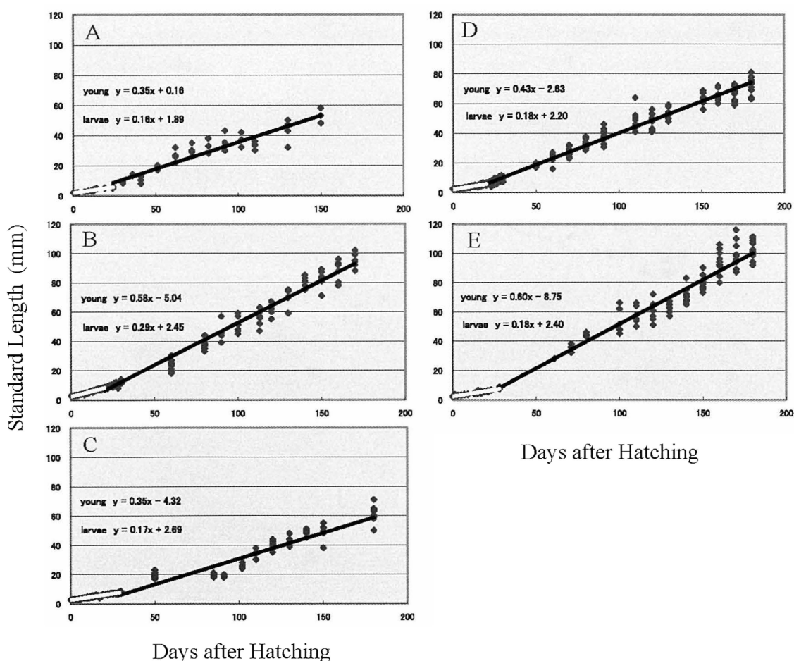
Fig. 4. Growth diagrams and growth regression lines (larvae, white lines; young fishes, black lines) of Takifugu niphobles (A), T. pardalis (B), T. poecilonotus (C), T. snyderi (D) and T. stictonotus (E).
