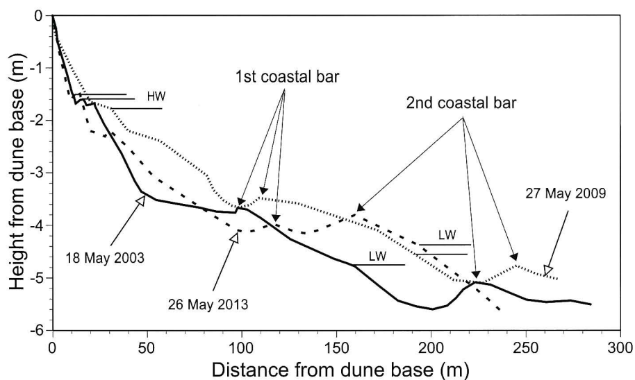
Fig. 2 Beach profiles at Kyoden site. Positions of 1st and 2nd coastal bars and sea levels at high (HW) and low (LW) waters were indicated.
