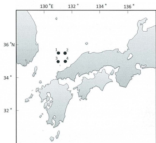
Fig. 1. Location of research area. Sea-surface and mid-water trawl, and conductivity-temperature-depth (CTD) measurements, at the filled circle.
