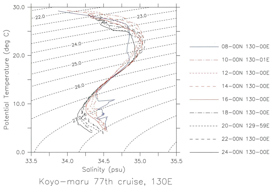
Fig. 4. Potential temperature-salinity relationships at the stations of every 2 degrees along 130°E during Koyo-maru 77th cruise.
