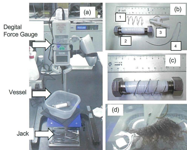
Fig. 2 Photographs showing the equipment used for adherence strength measurement. (a) shows a whole view of the equipment, (b) and (c) show the parts of improved clip in the present study, and (d) shows the clip with catching a blade of nori.
