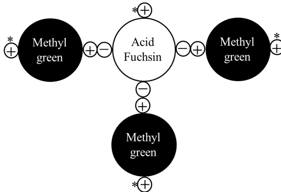
Fig. 3. Schematic illustration of the expected dye complex in basic neutral mixture (basic triacid stain). Combination of tribasic acid dye (acid fuchsin) and diacidic basic dye (methyl green). ⊕, acid group; ⊖, basic group. Astarisk indicates free group.
