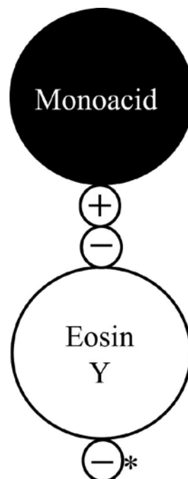
Fig. 1. Schematic illustration of the expected dye complex in Romanowsky's 4) and Pappenheim's 5) neutral mixture (triacid stain). Combination of dibasic acid dye (eosin) and monoacidic basic dye (methylen blue 4) or methylen azure 5) ). ⊕, acid group; ⊖, basic group. Astarisk indicates free group.
