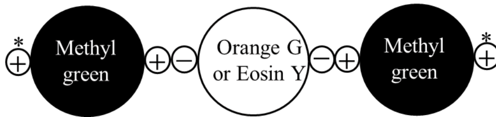
Fig. 2. Schematic illustration of the expected dye complex in basic neutral mixture (basic triacid stain). Combination of dibasic acid dye (orange G or eosin) and diacidic basic dye (methyl green). ⊕, acid group; ⊖, basic group. Astarisk indicates free group.
