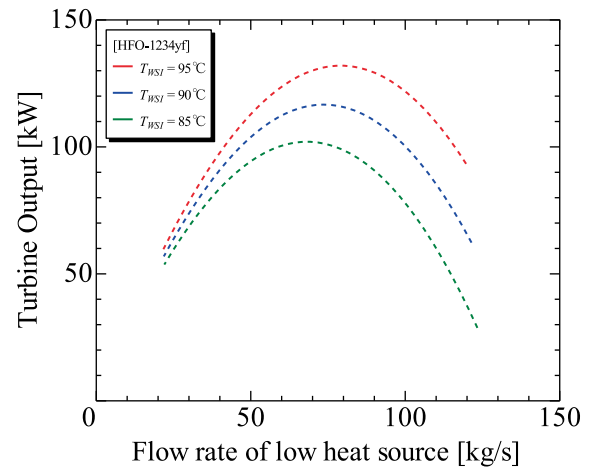
Fig. 10. The effect of the inlet temperature of high heat source at seafood processing plant when the maximum turbine output is optimal (HFO-1234yf).
