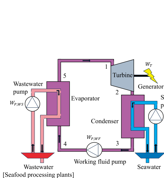
Fig. 1. Organic rankine cycle.
