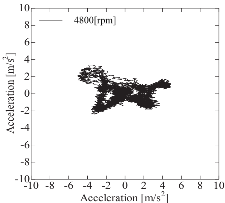
Fig.11 The trajectory of rotating shaft on X-Y plane (Rotating speed:4800 rpm)
