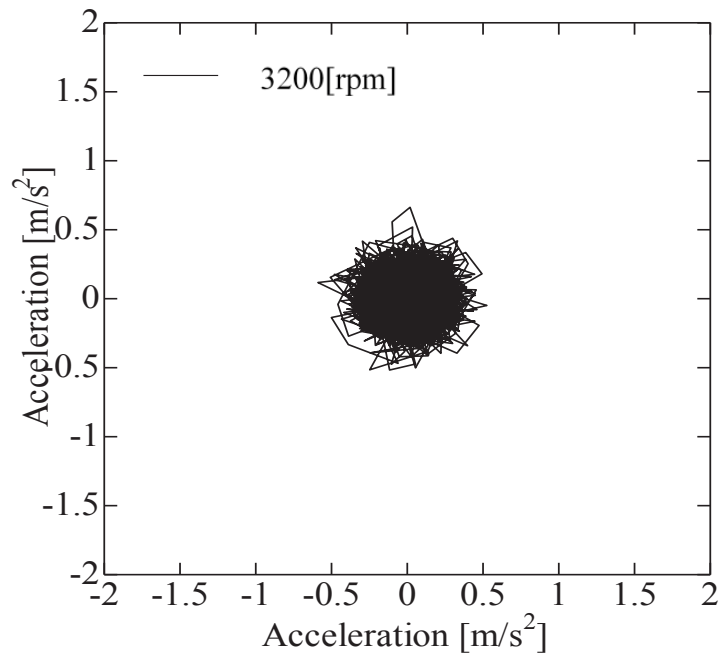
Fig.7 The trajectory of rotating shaft on X-Y plane (Rotating speed:3200 rpm)
