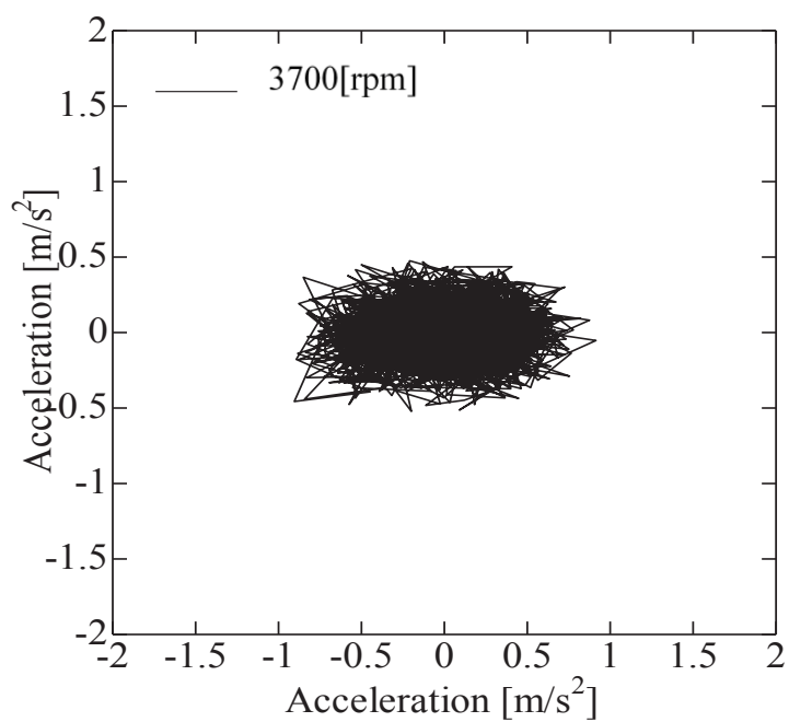
Fig.8 The trajectory of rotating shaft on X-Y plane (Rotating speed:3700rpm)
