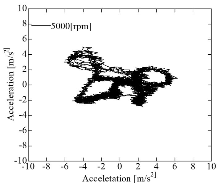
Fig.12 The trajectory of rotating shaft on the X-Y plane (Rotating speed:5000 rpm)
