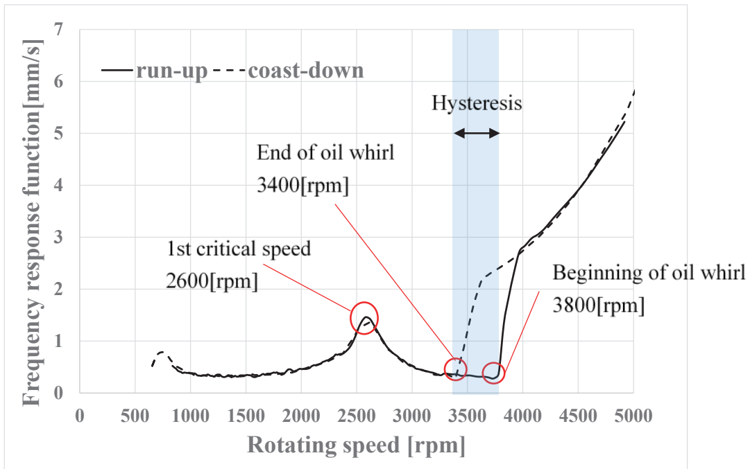
Fig.4 Result of frequency responses without unbalance (run-up and coast-down)
