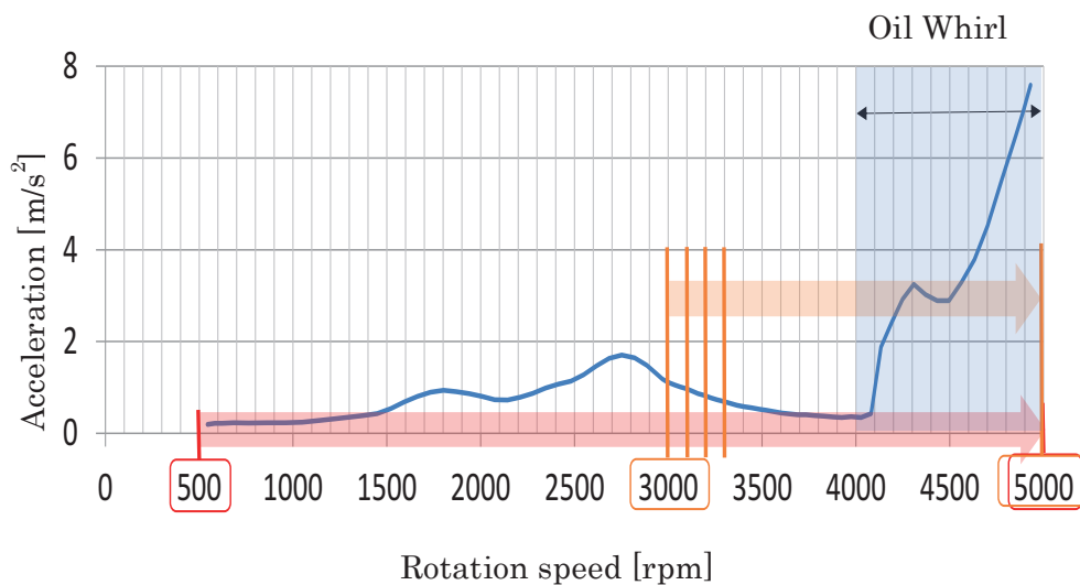
Fig.2 The frequency response of Oil Whirl generated by the sliding bearing test machine
