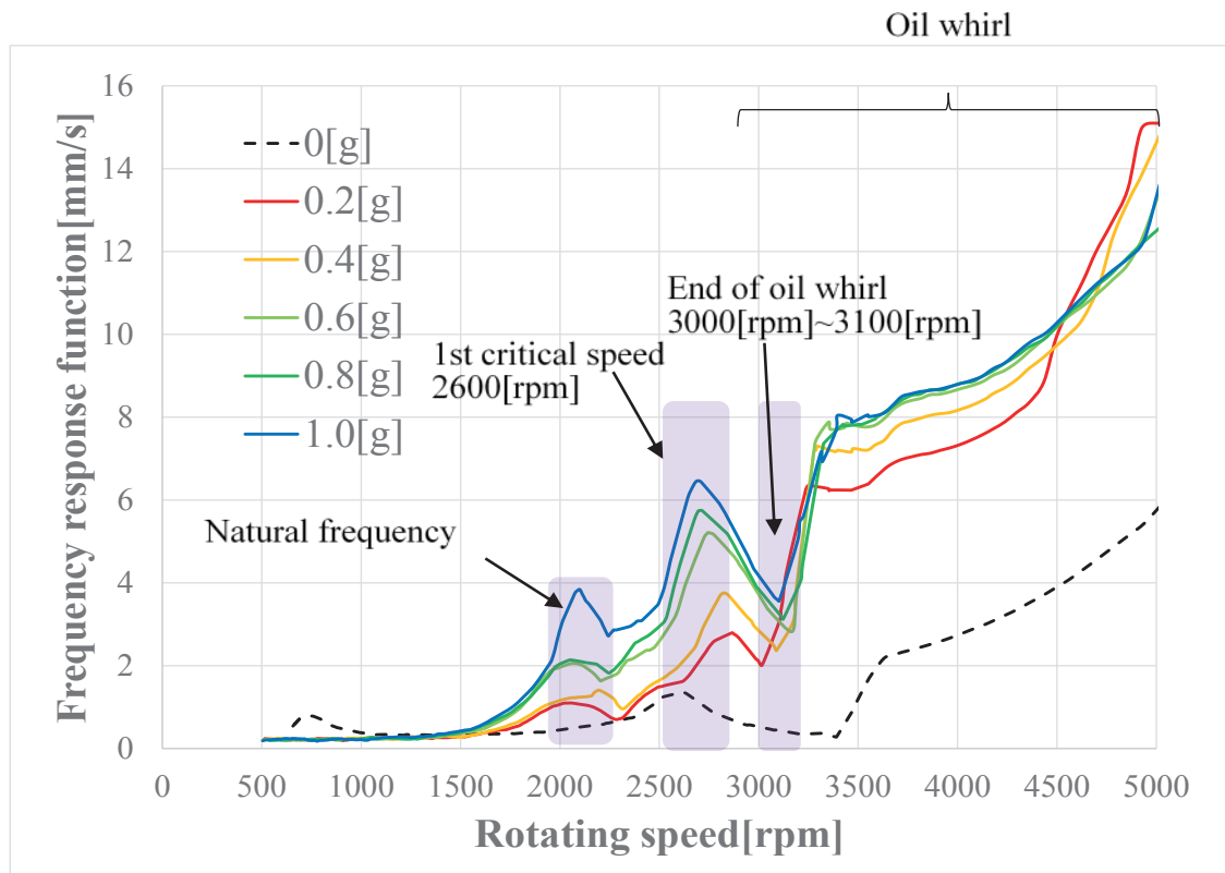
Fig. 6 Result of frequency response with unbalance (coast-down)
