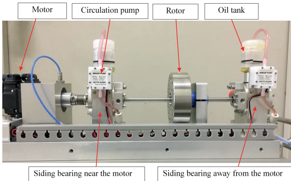
Fig.1 Sliding bearing test machine
