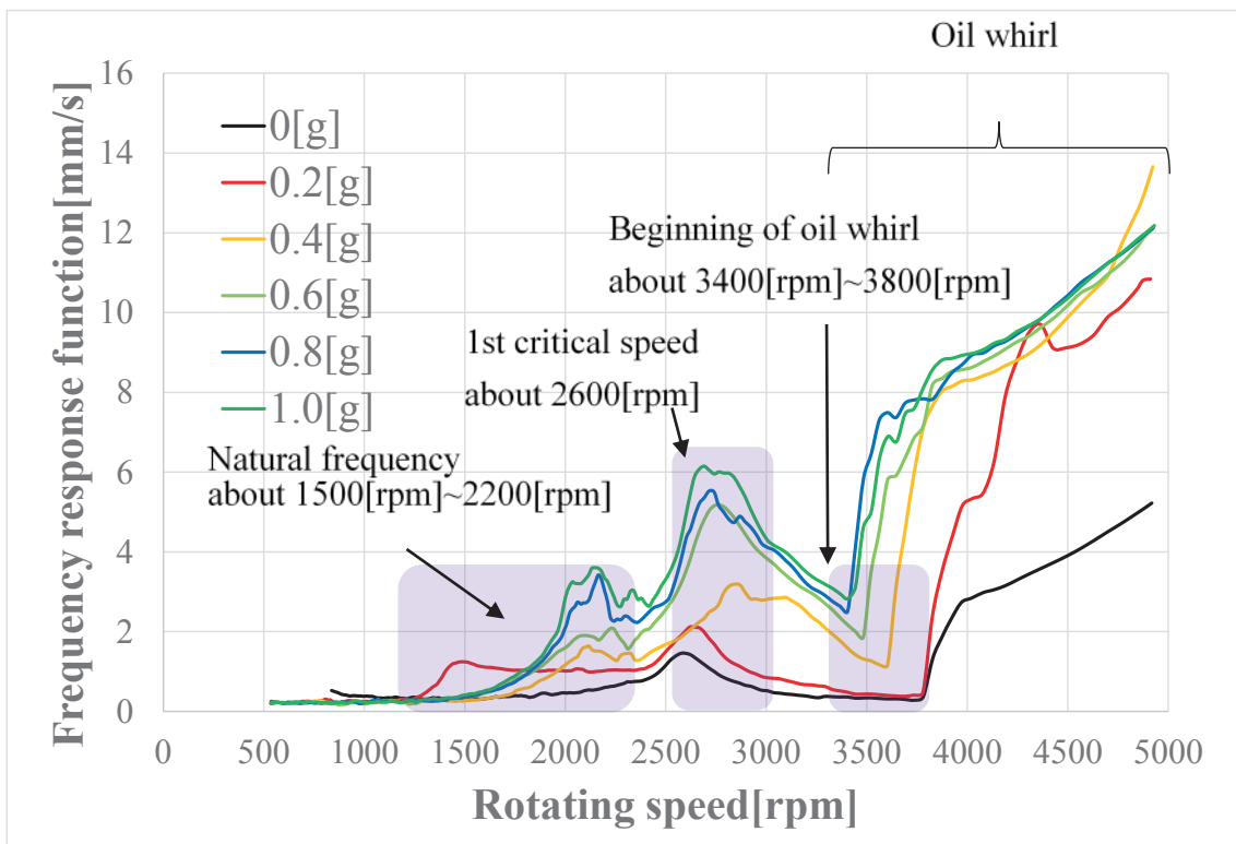
Fig.5 Result of frequency responses with unbalance (run-up)
